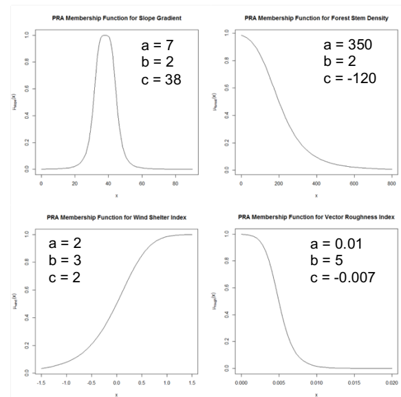
Figure 3: Cauchy membership functions for model parameters
