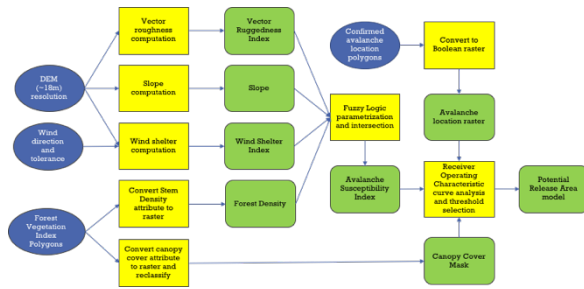
Figure 2: PRA model algorithm
