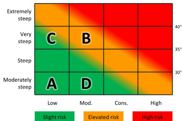
Figure 2: Slopes of Scenario 3 plotted on the Graphic Reduction Method chart.
